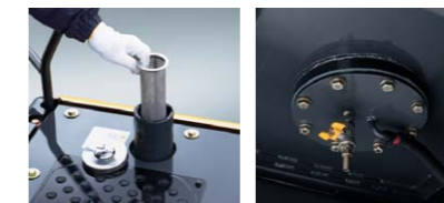
Stainless steel strainer Maintenance hole for cleaning
